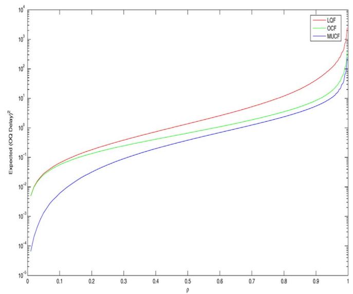
Fig. 8. Comparison of the logarithm of second moments of the output queued delays of different scheduling algorithms.
